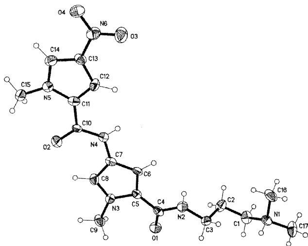
Figure 1 The structure of the cation in the title compound, (I), with displacement ellipsoids drawn at the 50% probability level for non-H atoms.
