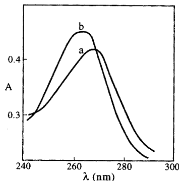
Fig. 4. Absorption spectra of the \text{Co}(\text{phen})_2\text{dppz}^{3+} -DNA system ( C_{\text{DNA}} = 16 \mu\text{M} , R_f = [\text{DNA}]/[\text{Co}] = 2 ) without light (a) and after irradiation at 254 nm for 20 min (b).
