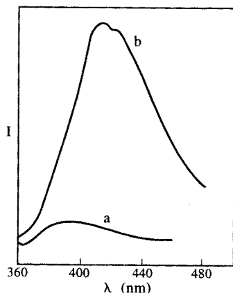
Fig. 3. Fluorescence spectra of \text{Co}(\text{phen})_2\text{dppz}^{3+} ( 50 \mu\text{M} ) in the absence (a) and presence (b) of DNA, R_f = [\text{DNA}]/[\text{Co}] = 44 . Sample excitation was at 330 nm.
