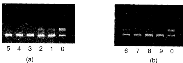
Fig. 5. (A) Cleavage of pBR 322 DNA in the presence of \text{Co}(\text{phen})_2\text{dppz}^{3+} and light. DNA alone (lane 0), the concentration of \text{Co}(\text{phen})_2\text{dppz}^{3+} was 2.5, 5, 7.5, 10, 15 \mu\text{M} (lanes 1-5) (B) pBR 322 DNA was incubated with \text{Co}(\text{phen})_2\text{dppz}^{3+} (10 \mu\text{M} ) and irradiated for 5, 10, 20, 30 min (lanes 6-9).
