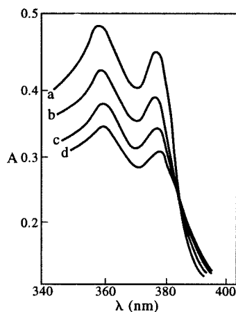
Fig. 2. Absorption spectra of Co(phen) 2 dppz 3+ (10 μM) in the absence and presence of DNA. R_t = [\text{DNA}]/[\text{Co}] = 0, 0.5, 1, 2 for a–d, respectively.
